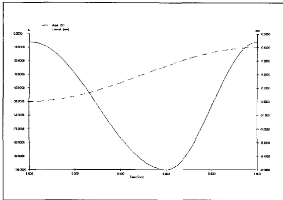
Fig. 1. Chewing simulation
