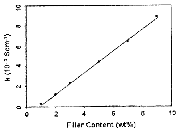
Figure 7. Conductivity of PC/PANI nanocomposite as a function of PANI nanofiller content.
