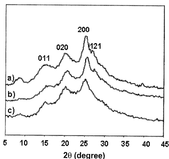
Figure 6. XRD patterns of PANI nanoparticles prepared at (a) 3 °C, (b) 25 °C, and (c) 60 °C using OTAB.
