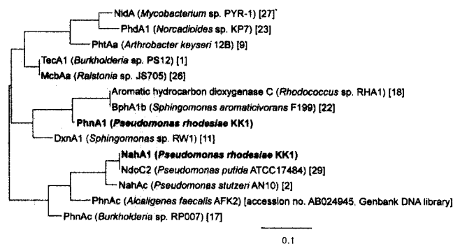
Fig. 2. Phylogenetic tree of Rieske iron-sulfur motif sequences of putative dioxygenases in strain KK1.
