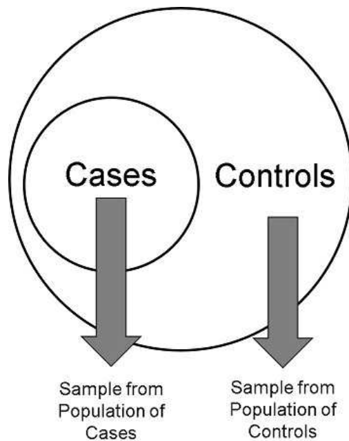
Figure 1.1 Case-control sampling design
