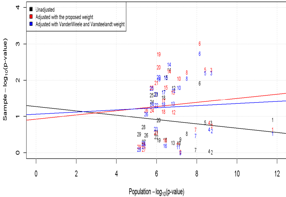
Figure 3.1 Comparison of p-values (population-based p-value threshold < 1E-05) using unadjusted samples (black-colored), adjusted samples with the proposed weight (red-colored), and adjusted samples with VanderWeele and Vansteelandt weight (blue-colored)
