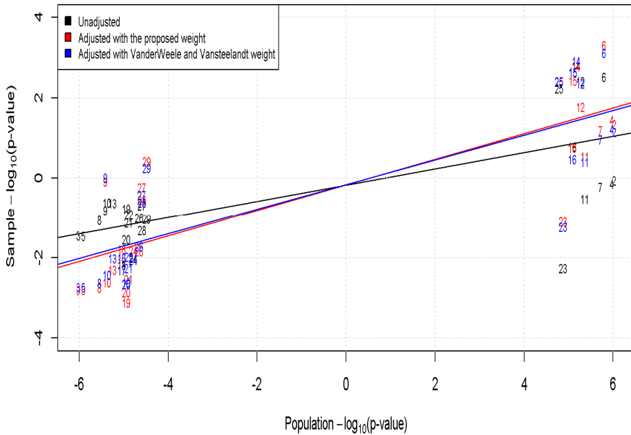
Figure 3.2 Comparison of test statistics (population-based p -value threshold < 1E-05 ) using unadjusted samples (black-colored), adjusted samples with the proposed weight (red-colored), and adjusted samples with VanderWeele and Vansteelandt weight (blue-colored)
