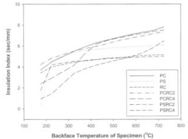
Fig. 11 Insulation Index of Carbon Fabric Composites.
