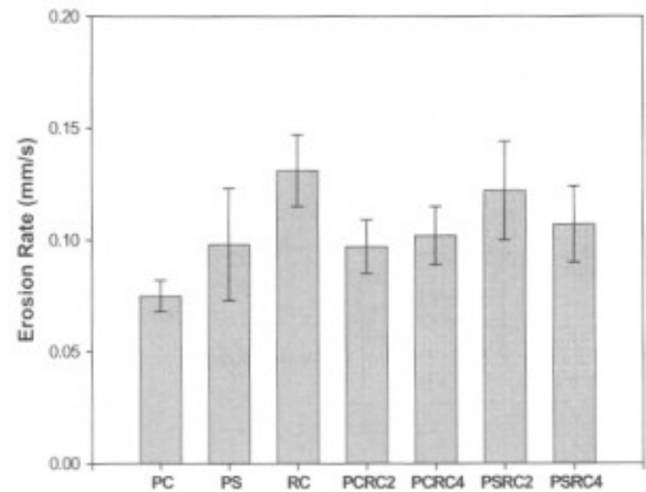
Fig. 10 Erosion Rate of Carbon Fabric Composites.
