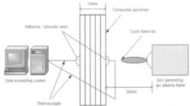
Fig. 4 Schematic Illustration of Apparatus for Ablation Test using an Arc Plasma Torch.
