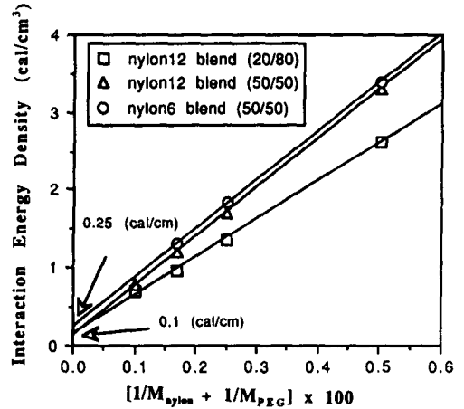
Fig. 4. The Massa's plot showing the change of interaction energy density for blends of nylon 12 and nylon 6 with PEG having various molecular weights.
