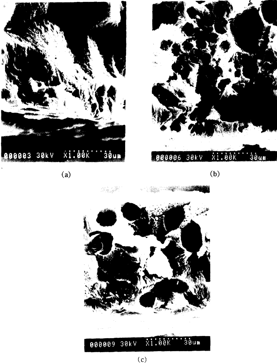
Fig. 7. SEM photographs of the cross section of a membrane prepared from blends of (a) nylon 12/PEG 200, (b) nylon 12/PEG 400, (c) nylon 12/PEG 600 for quenching depth of 50°C ( \times 1000 ).
