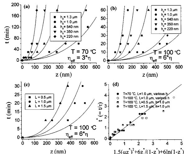
FIG. 3. Comparison of the theoretical model with the experimental data at (a) 70 °C and (b) 100 °C for various film thicknesses for the strip width of 2 μm ( L = 1 \mu\text{m} ). (c) Effect of channel width on the rate of capillary rise at 100 °C for the film thickness of 1.0 μm. (d) A generalized diagram as a function of the dimensionless time and length.
