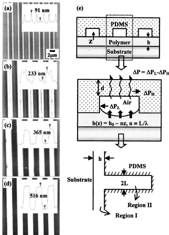
FIG. 1. (a)–(d) Planar and cross-sectional views of AFM profiles for the 2 μm line-and-space pattern as a function of annealing time [(a) 10, (b) 30, (c) 60, and (d) 180 min] at 70 °C for the film thickness of 1.0 μm. (e) Schematic illustration of the capillary rise into permeable microcavities and a series of channel resistances.
