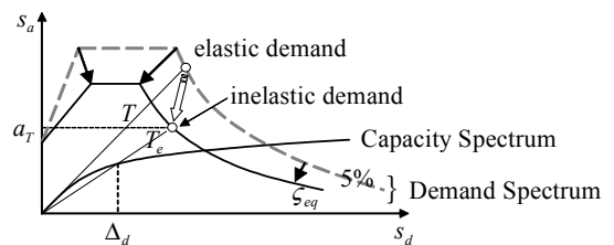
Fig. A1 Reduced strength demand(CSM)
