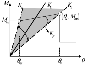
Fig. 4 Admissible range of secant stiffness
