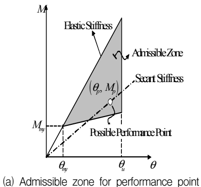
Fig. 2 Determination of inelastic strength and deformation of the member using secant stiffness
