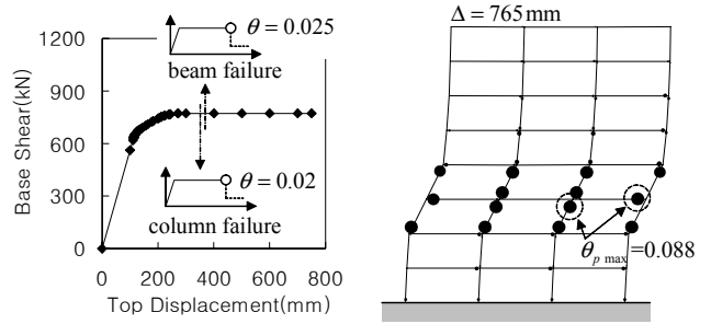
Fig. 8 Existing elastic design for equivalent static seismic load
