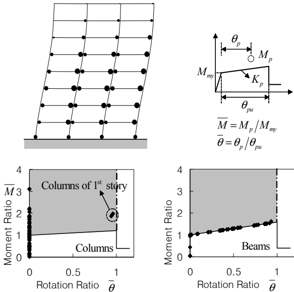
Fig. 11 Performance-based design results: CP
