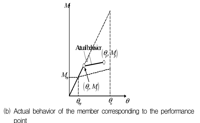
Fig. 2 Determination of inelastic strength and deformation of the member using secant stiffness
