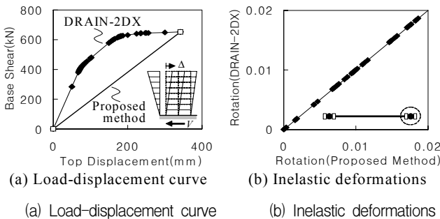
Fig. 12 Verification of the proposed method (CP)
