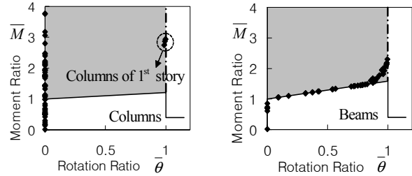
Fig. 9 Force-based design results : CP
